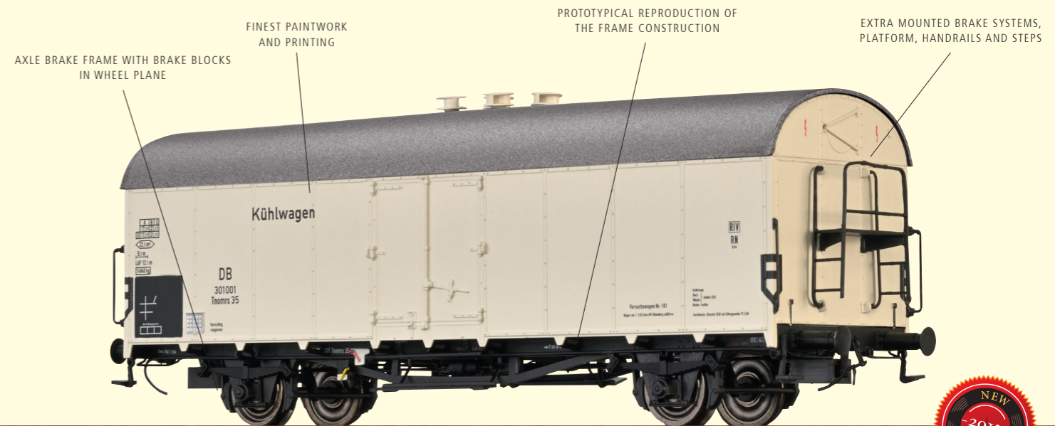
Refrigerator Car Tnomrs 35 DB Road no. 301 001
